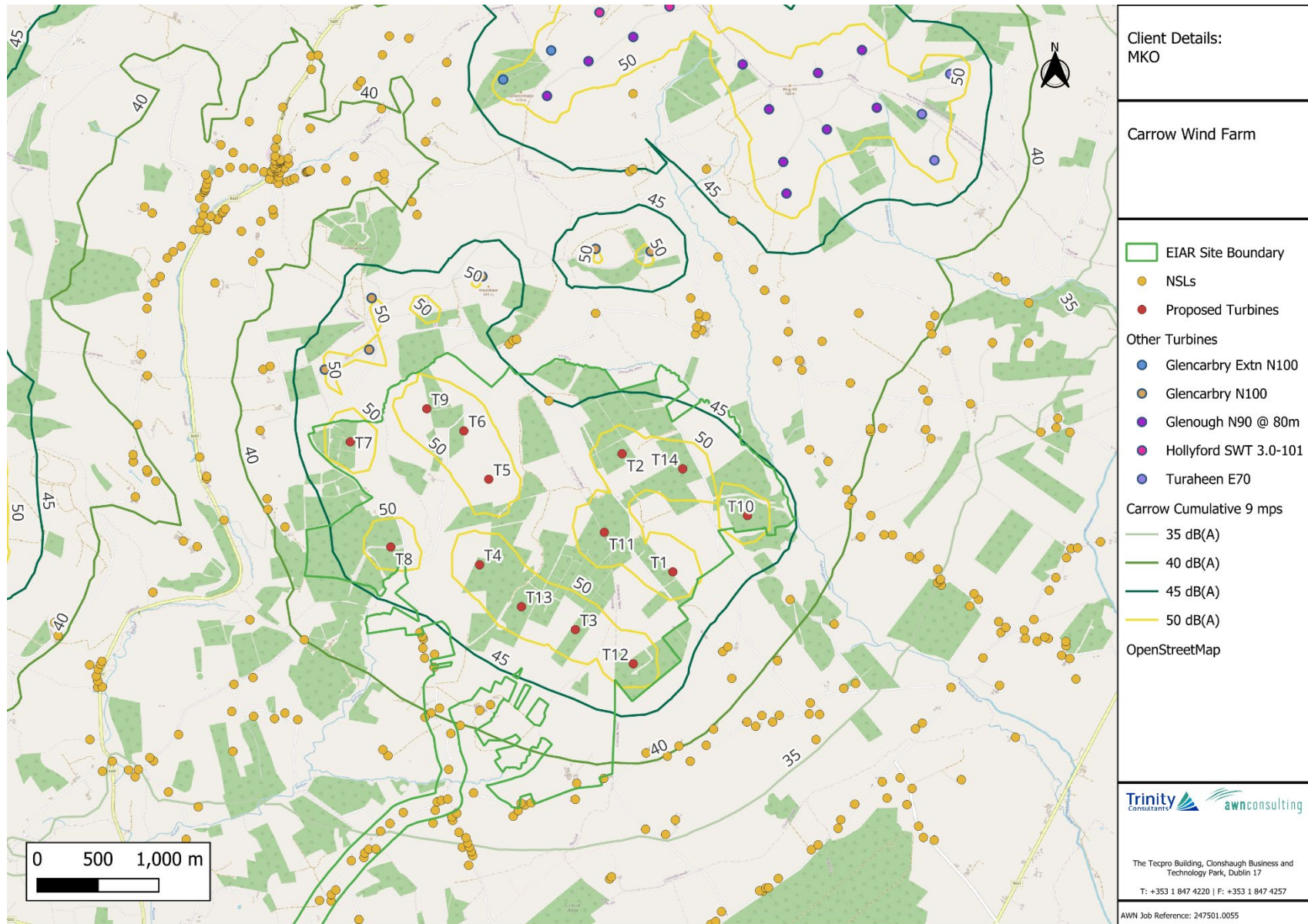
Figure 12-8-1. Predicted Cumulative Noise Contours Overall
