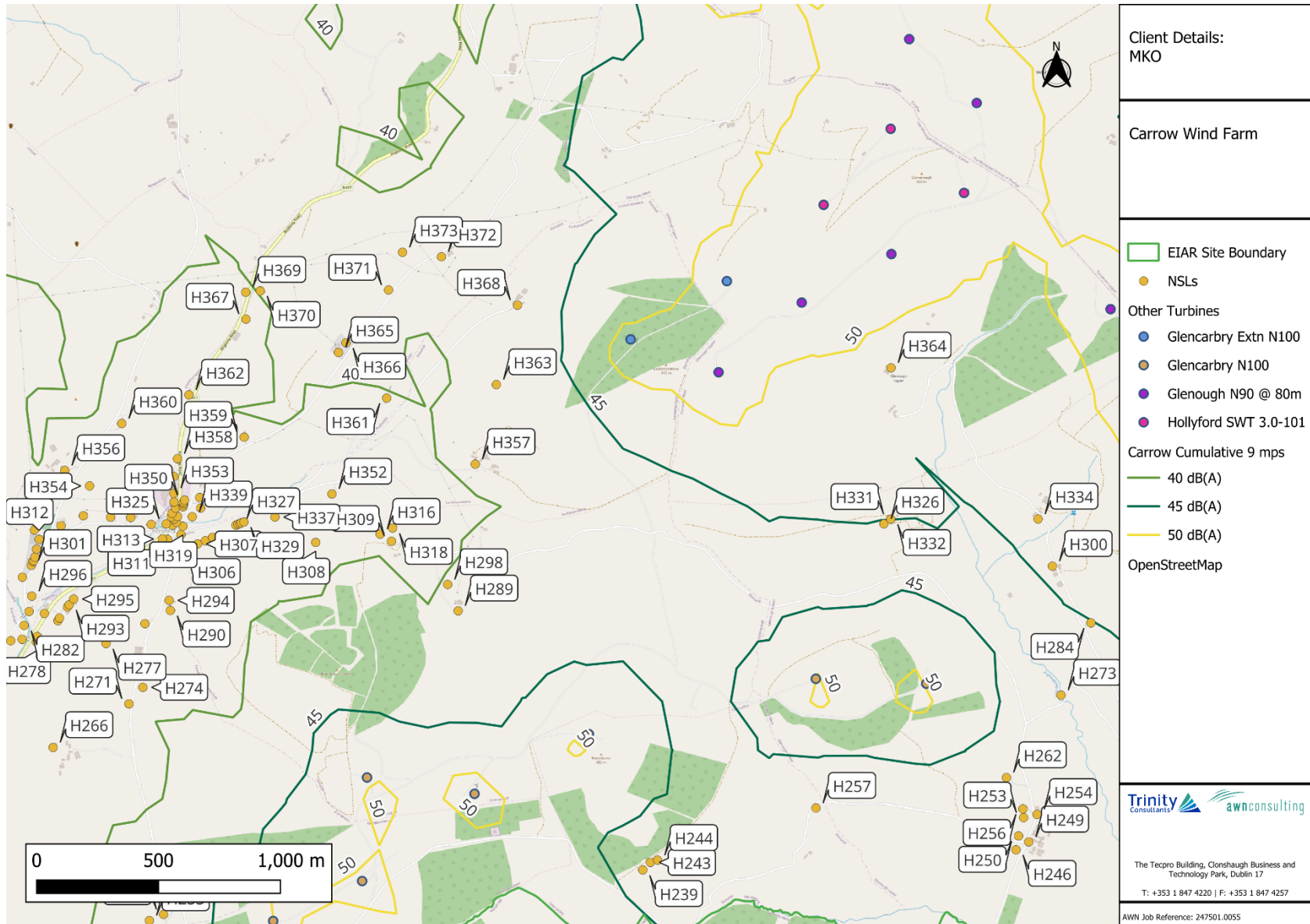
Figure 12-8-5. Predicted Cumulative Noise Contours Detail 5 of 5
