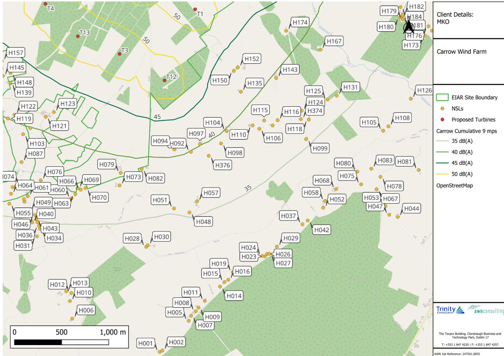
Figure 12-8-4. Predicted Cumulative Noise Contours Detail 3 of 5
