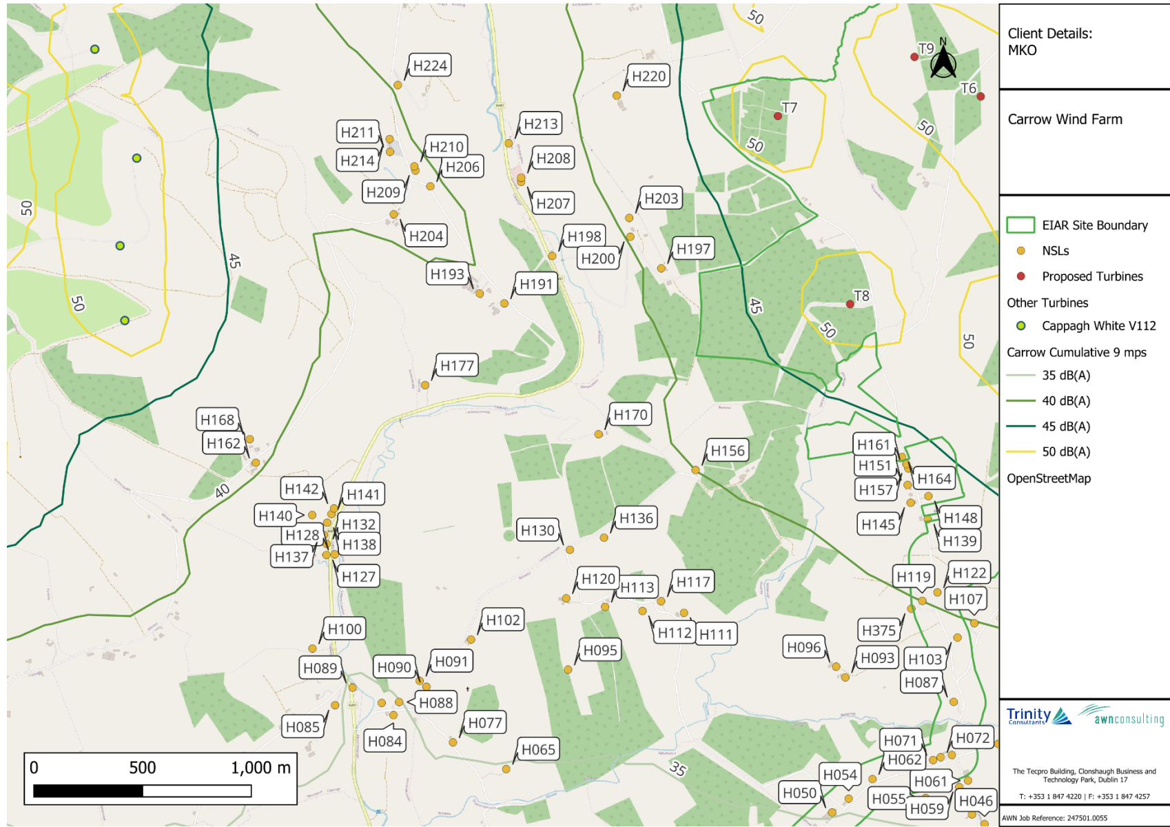
Figure 12-8-3. Predicted Cumulative Noise Contours Detail 2 of 5
