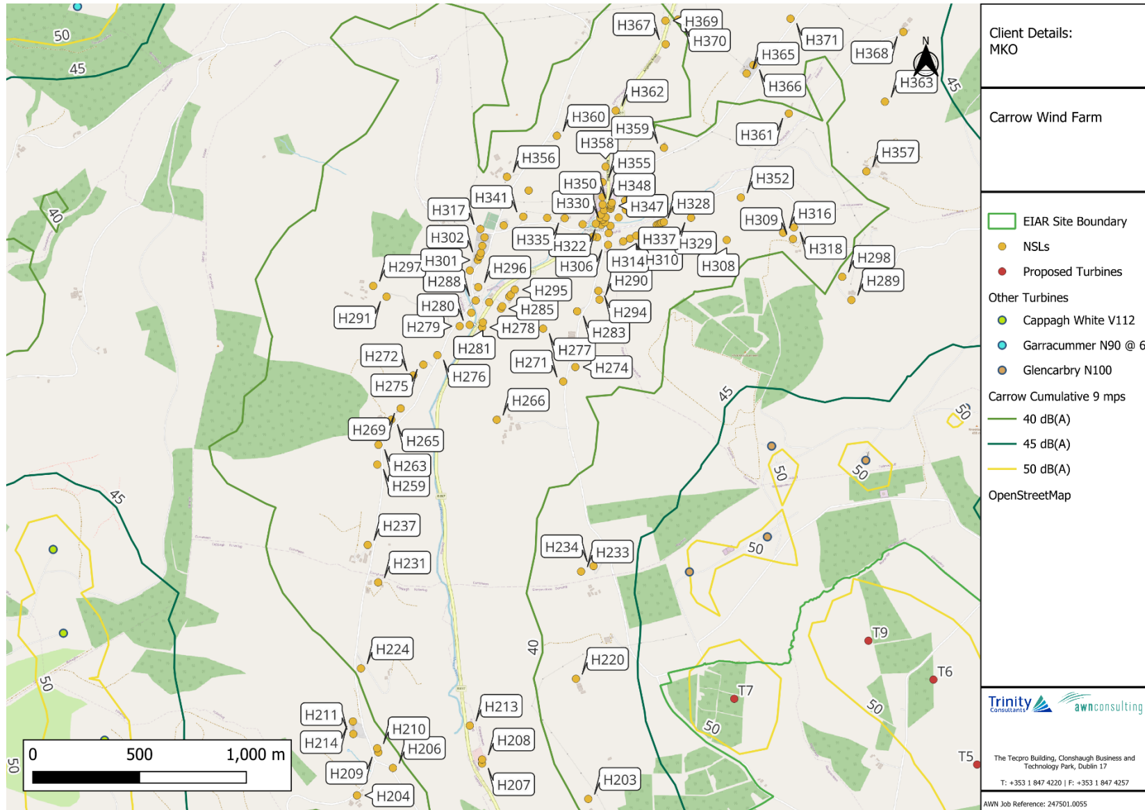
Figure 12-8-2. Predicted Cumulative Noise Contours Detail 1 of 5
